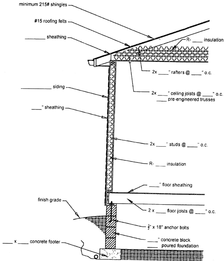
Typical Wall Section through Addition
