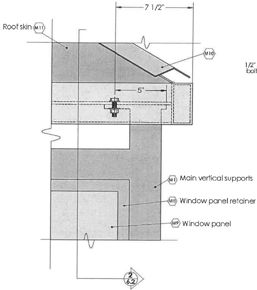
1 10 ROOF ASSEMBLY SIDE DETAIL Scale: 3"=1'
