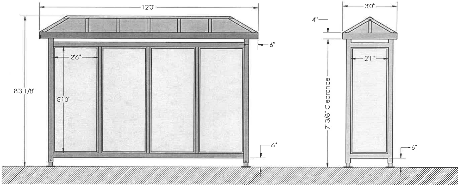
2 3 SIDE FRONT VIEW Scale: 1/2"=1'
