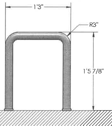
3 12 SIDE VIEW Scale: 1 1/2"=1'
