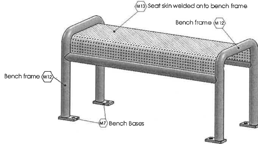
4 12 ISOMETRIC VIEW Scale: 1 1/2"=1'
