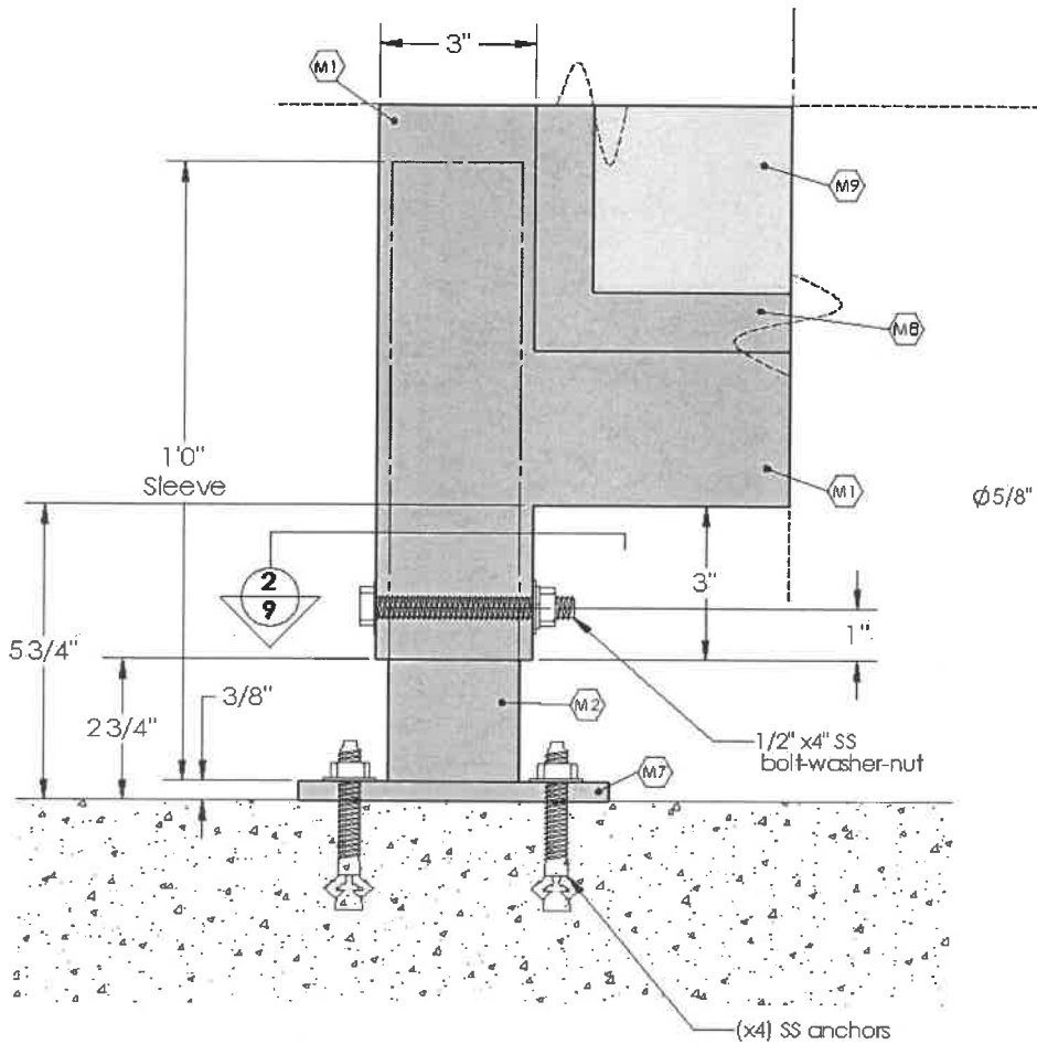
1 9 SLEEVE-LEG DETAIL Scale: 4"=1'
