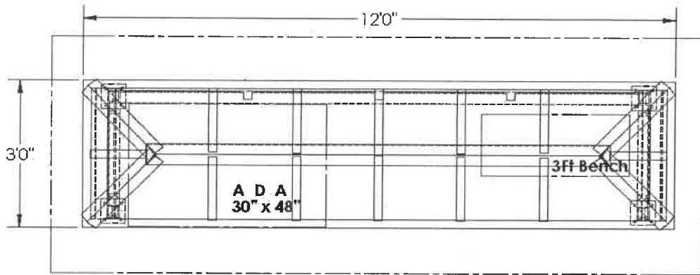
3 3 SHELTER TOP VIEW Scale: 1/2"=1'
